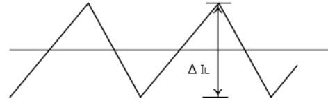
Figure 46. Inductor Current
